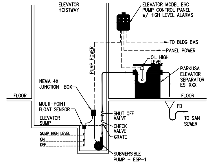
① ELEVATOR SUMP DETAIL NOT TO SCALE (ABOVEGROUND SEPARATOR)
