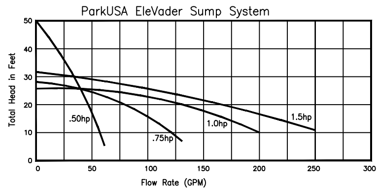
④ PUMP CURVE NOT TO SCALE
