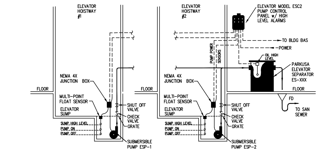
① ELEVATOR SUMP ESP-1 & 2 DETAIL NOT TO SCALE (ABOVEGROUND SEPARATOR)
