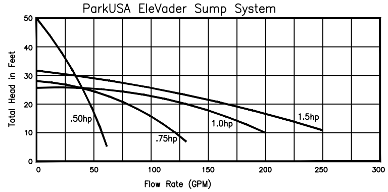
④ PUMP CURVE NOT TO SCALE
