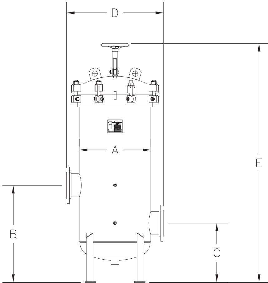
ParKlear™ Cartridge Filter Vessel Sizes
