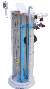
Grinder Pump
